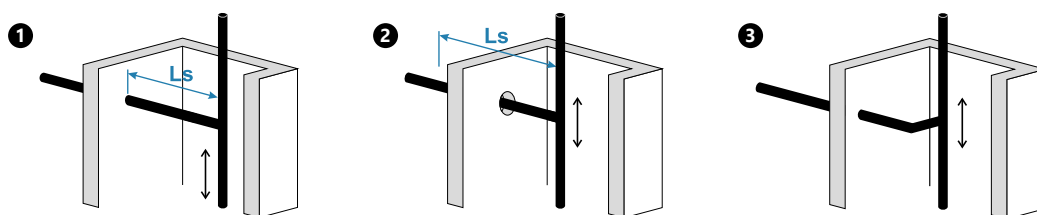
Ensuring a flexible arm on riser branch-offs in installation shafts (examples)
