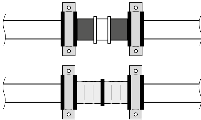
Example of execution of a fixed point on a straight section of a KAN-therm ultraLINE, ultraPRESS, system pipeline
