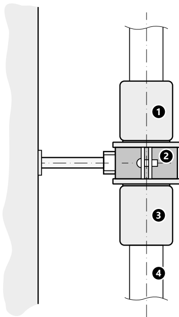
Example of execution of a fixed point on a straight section of a KAN-therm PP Green system pipeline
