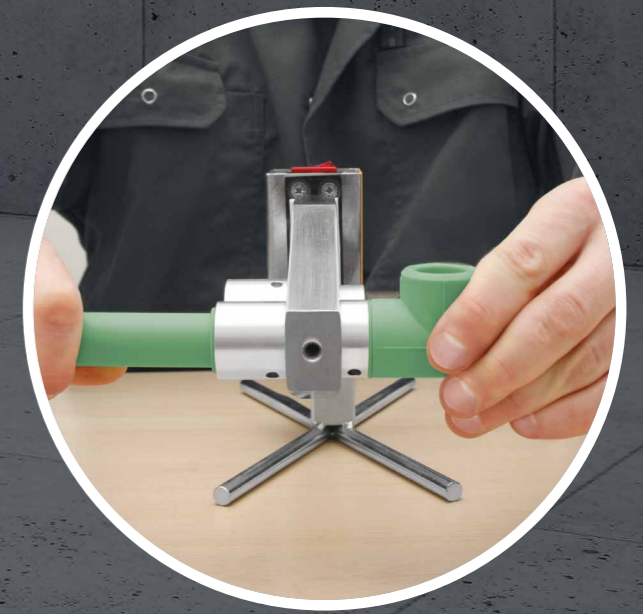
04 Heating the pipe and fitting.
