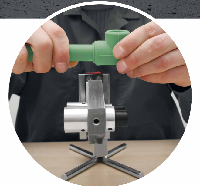
06 Fixing and cooling down the joint.
