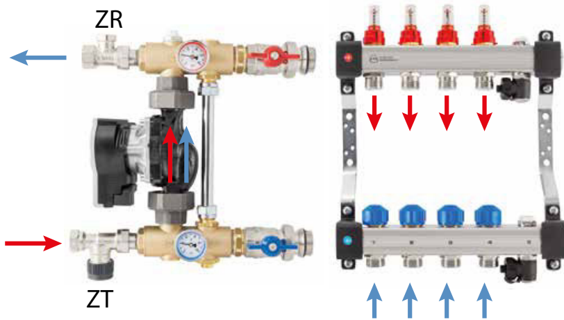
Fig. 56. Constant-value pump group with UFST manifold – flow directions.
